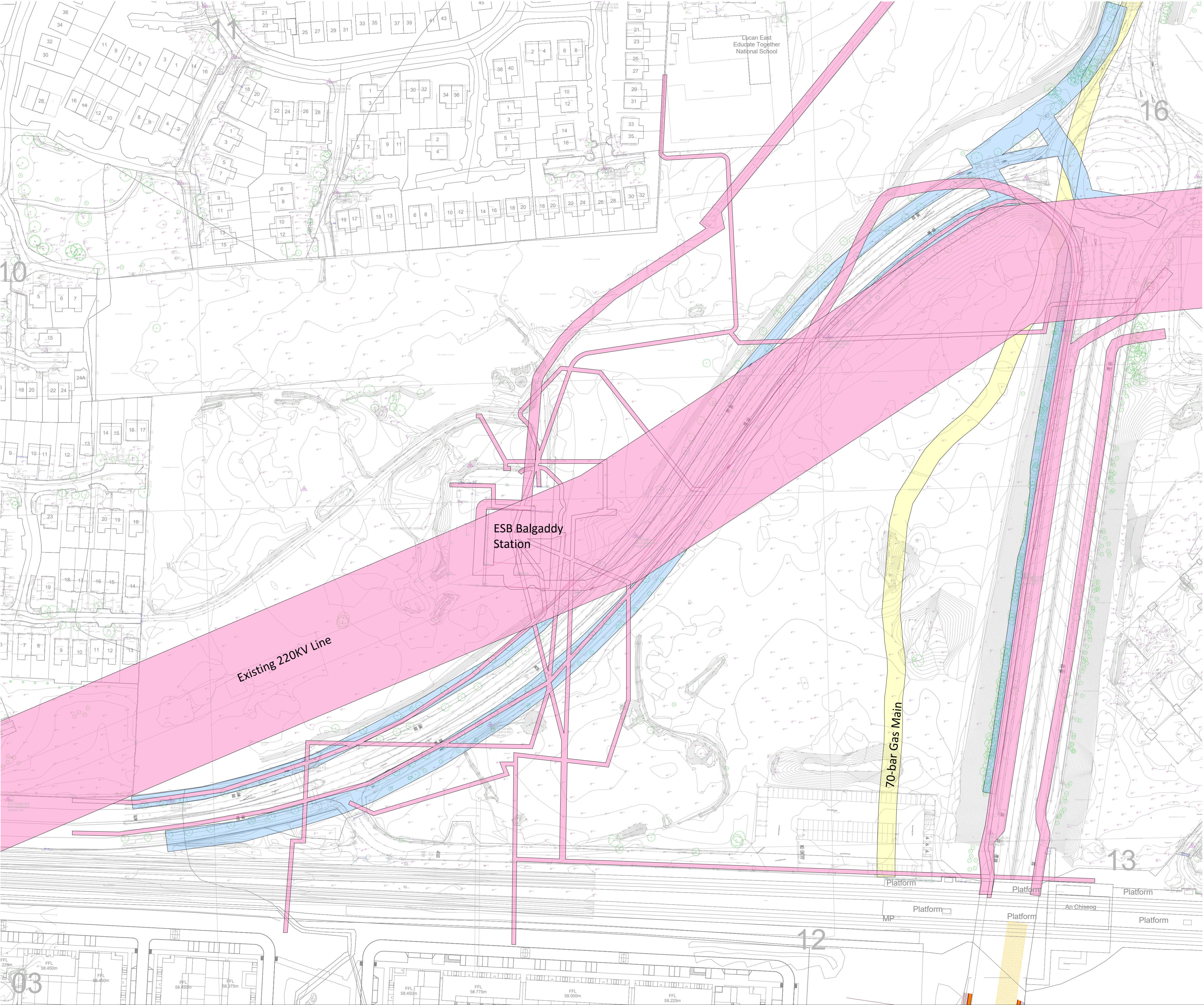
Site 3 Existing Services + Survey Layout
